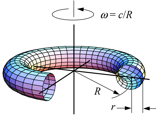
Figure 1: The Spinning Ring Model of the Electron
